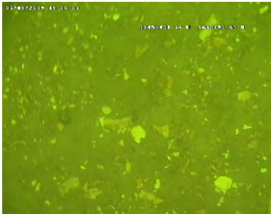
Photo B-5: Station #9 Unnamed Shoal B at a depth of 55 ft with no surface bedforms and high shell content.
