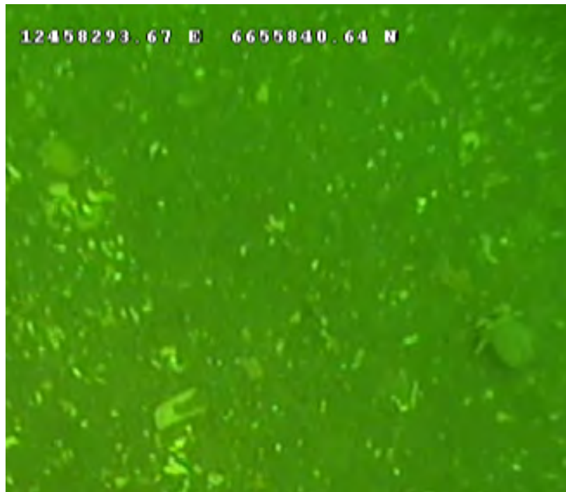
Photo B-16: Station #29 from Unnamed Shoal B at a depth of approximately 66 ft. Hermit crab ( Pagurus spp.) located in lower right quadrant.
