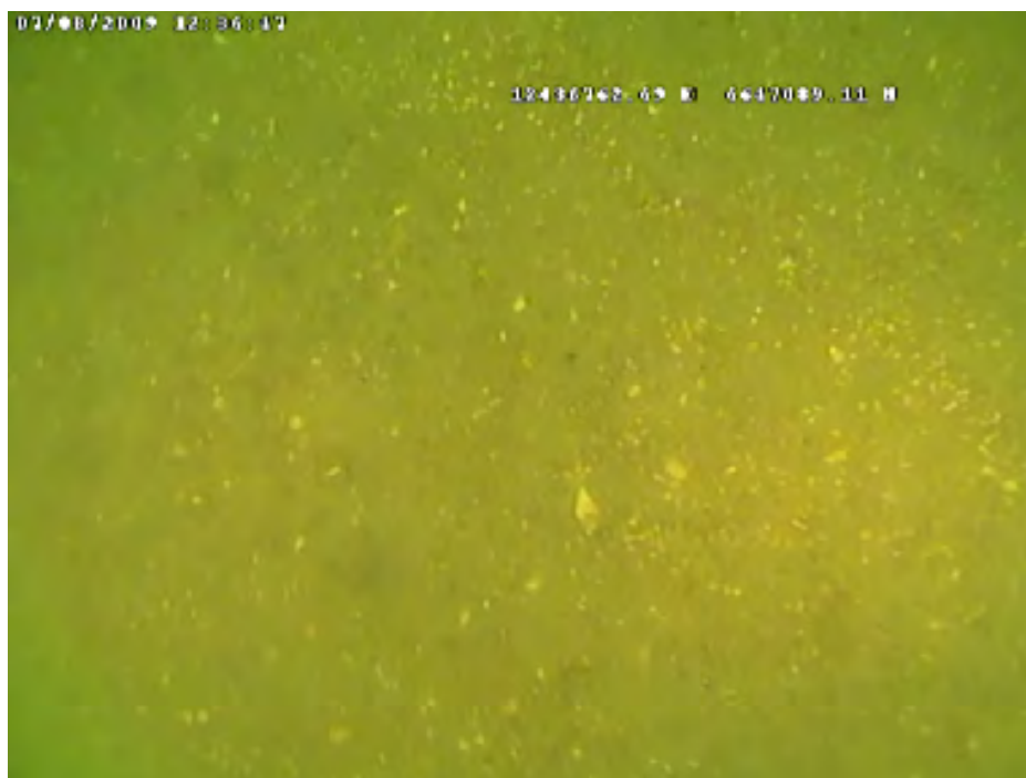
Photo A-8: Station #31 from Unnamed Shoal A at a depth of 50 ft with a lack of surface bedforms and low shell content.
