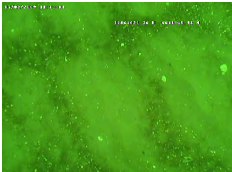
Photo B-18: Station #35 from Unnamed Shoal B at a depth of approximately 63 ft with defined bedforms and organic material concentrated in troughs.
