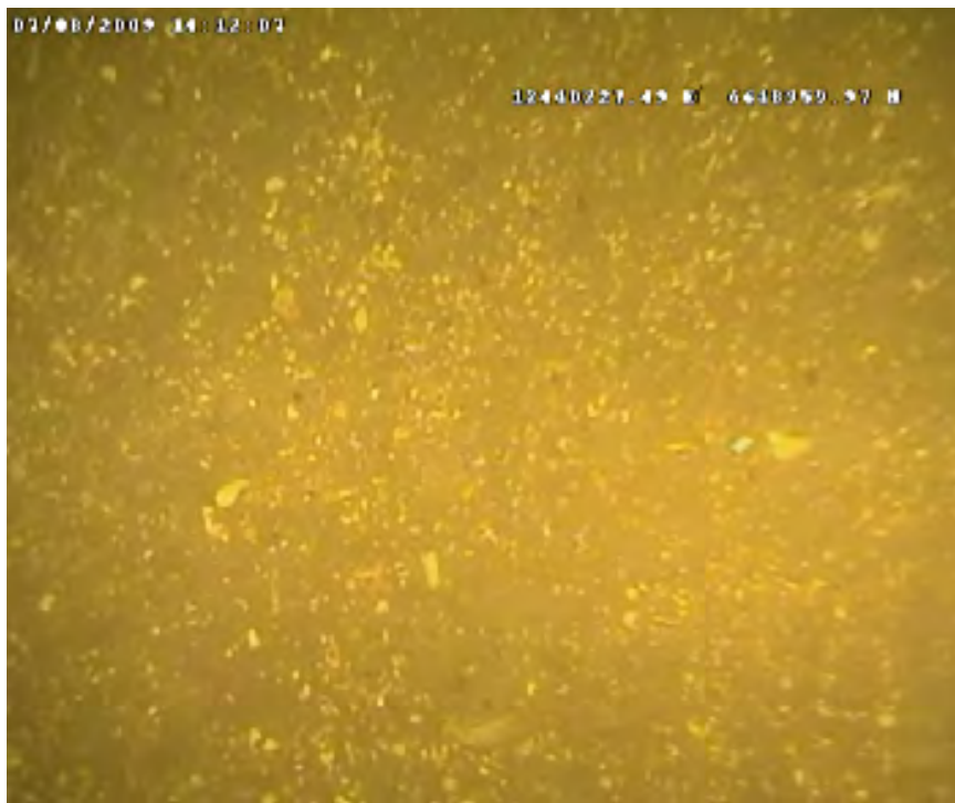
Photo A-6: Station #17 from Unnamed Shoal A at a depth of 64 ft with a high shell content and lack of surface bedforms.
