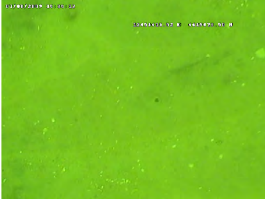
Photo B-2: Station #2 Unnamed Shoal B at a depth of 42 ft with well-defined ripple marks and low shell content characteristic of stations on shoal crest.
