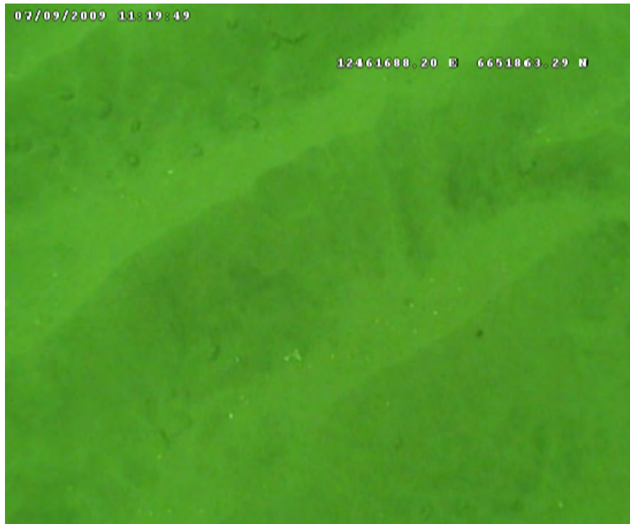
Photo B-11: Station #20 from Unnamed Shoal B at a depth of approximately 45 ft depicting well-defined ripple marks and low shell content.
