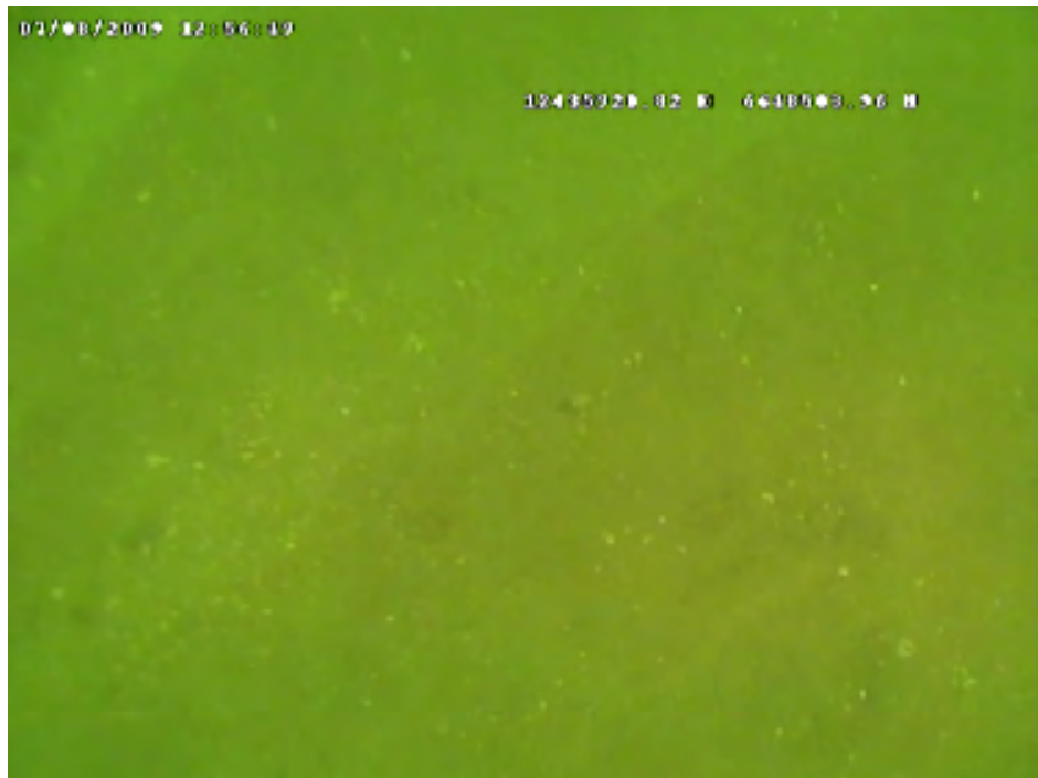
Photo A-9: Station #36 from Unnamed Shoal A at a depth of 42 ft with ripple marks and low shell content.
