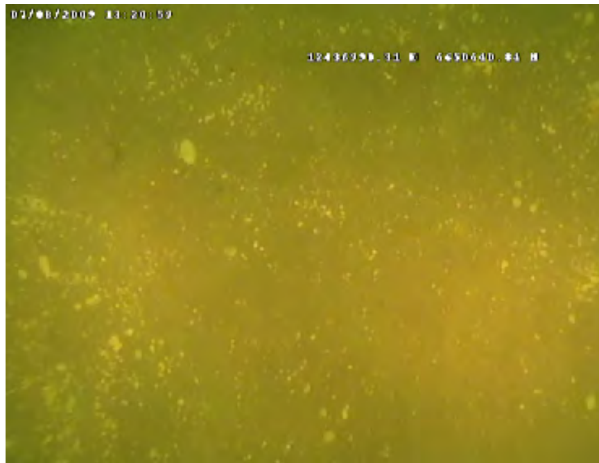
Photo A-6: Station #17 from Unnamed Shoal A at a depth of 64 ft with a high shell content and lack of surface bedforms.
