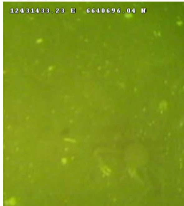
Photo A-8: Station #31 from Unnamed Shoal A at a depth of 50 ft with a lack of surface bedforms and low shell content.
