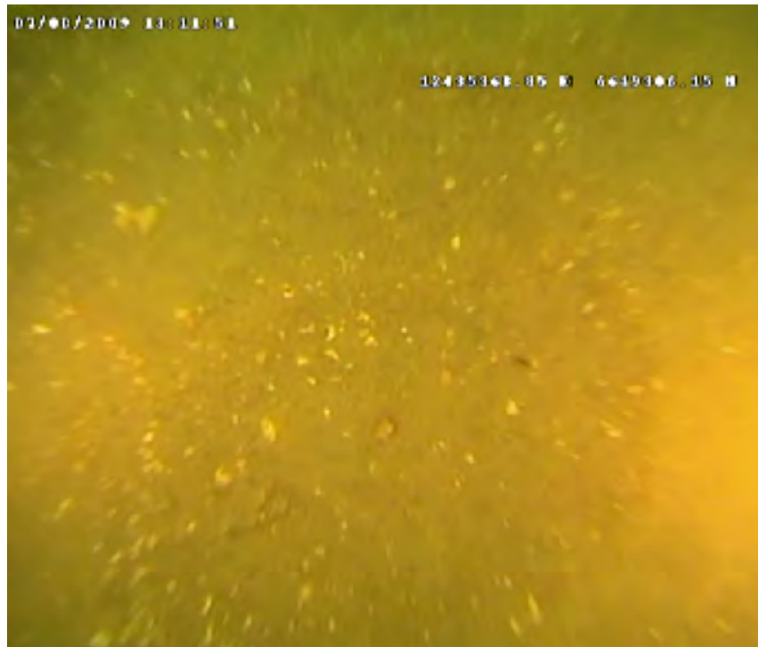
Photo A-4: Station #14 from Unnamed Shoal A at a depth of 53 ft with a lack of surface bedforms.
