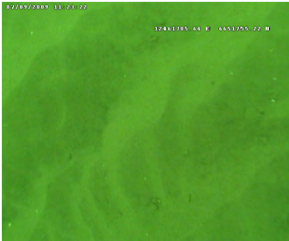
Photo B-12: Station #20 from Unnamed Shoal B at a depth of approximately 45 ft with well-defined ripple marks and low shell content.
