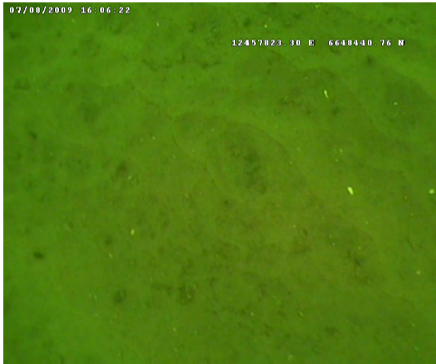
Photo B-19 : Station #39 from Unnamed Shoal B at a depth of approximately 56 ft with defined bedforms and low shell content.
