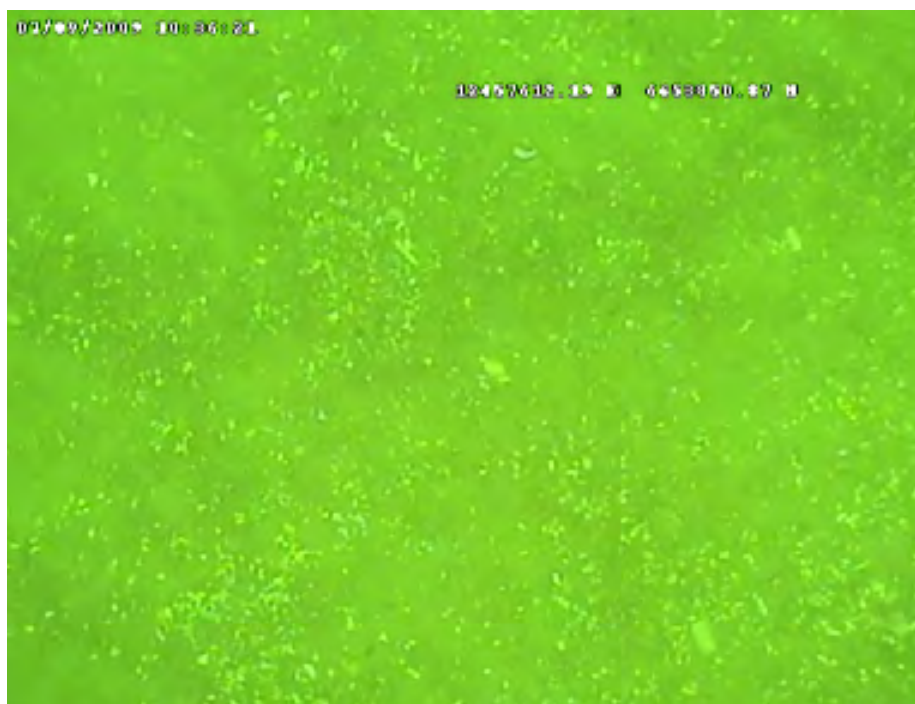
Photo B-8: Station #12 Unnamed Shoal B at a depth of 58 ft with lack of surface bedforms and high shell content.
