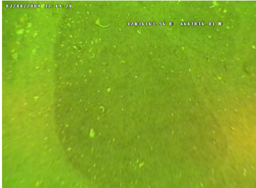
Photo A-4: Station #14 from Unnamed Shoal A at a depth of 53 ft with a lack of surface bedforms.
